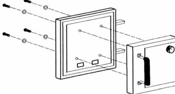
Fig. 4 – Door/Handle/Thermostat Assembly
