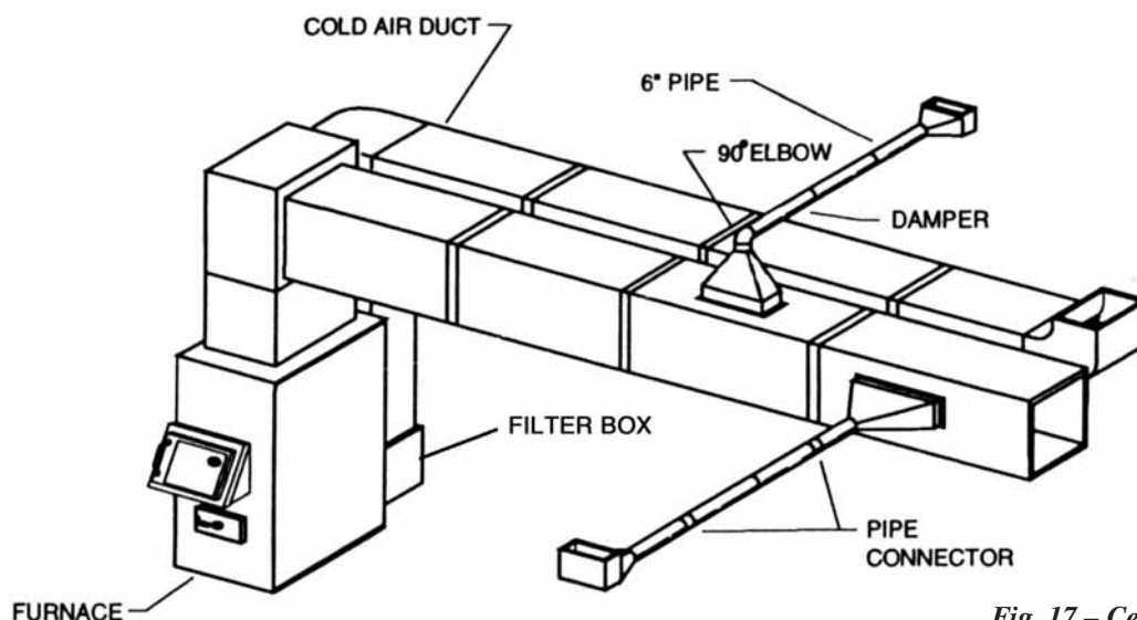
Fig. 17 – Central Installation
