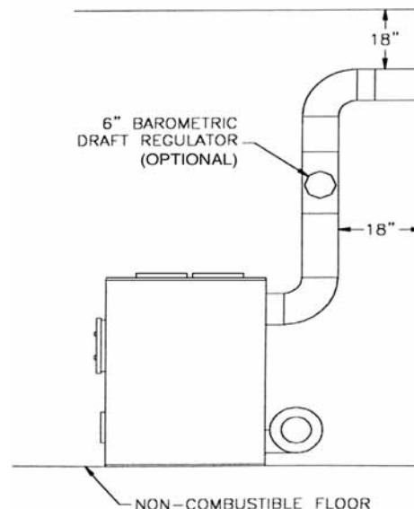
Fig. 2 – SIDE VIEW
