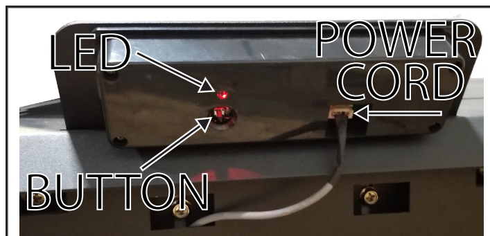
Figure 16 Display Panel Back (PSBF66W Shown)
