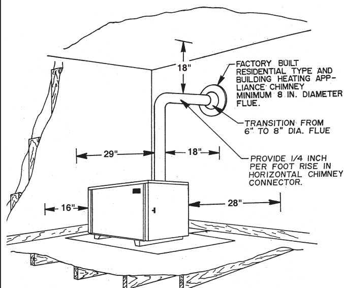
FIGURE 2 - MINIMUM CLEARANCES TO COMBUSTIBLES
