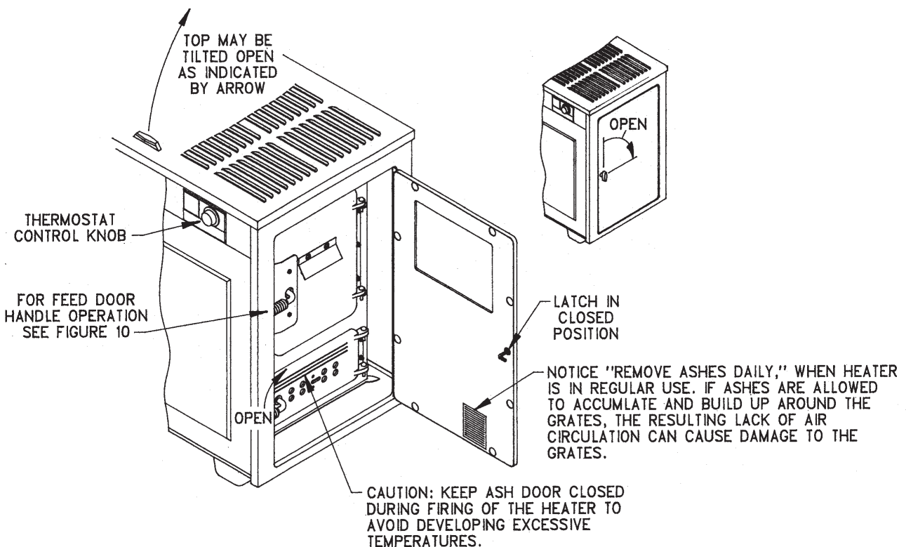
FIGURE 9 - HEATER OPERATION INFORMATION
