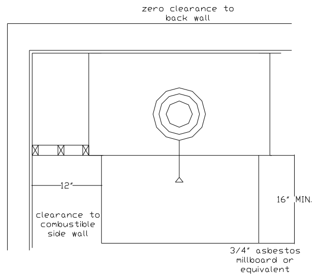
FIGURE 2 - FREESTANDING CLEARANCES (Top View)
