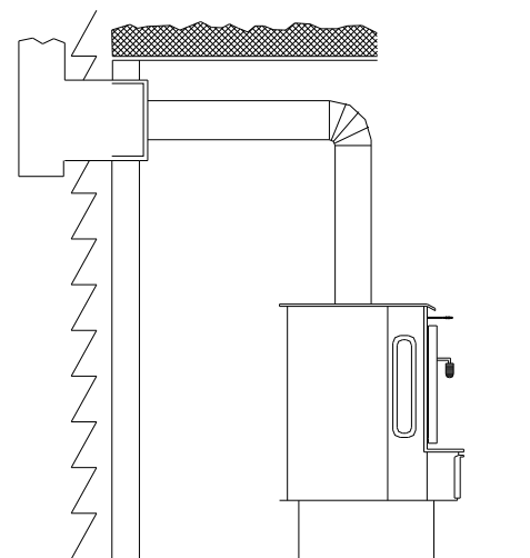
FIGURE 9 - INSTALLATION INTO A FACTORY BUILT CHIMNEY
