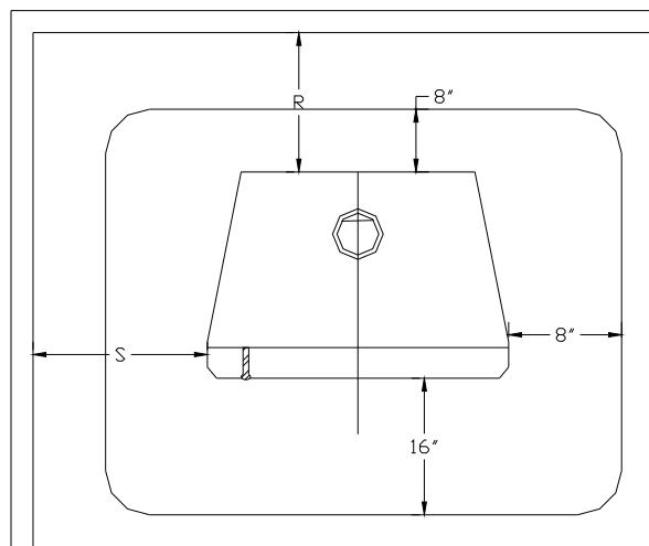
FIGURE 6 CLEARANCE TO COMBUSTIBLES
