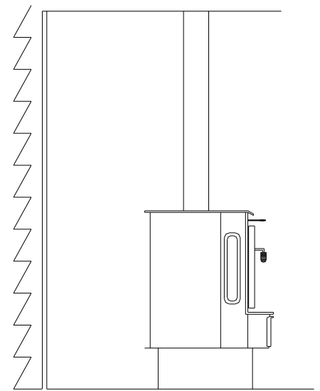
FIGURE 8 - INSTALLATION INTO A MASONRY FLUE
