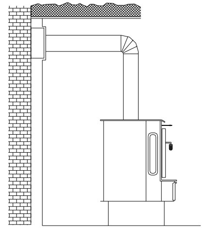
FIGURE 8 - INSTALLATION INTO A MASONRY FLUE
