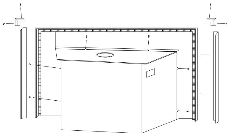
FIGURE 11 FRONT EDGE BRASS
