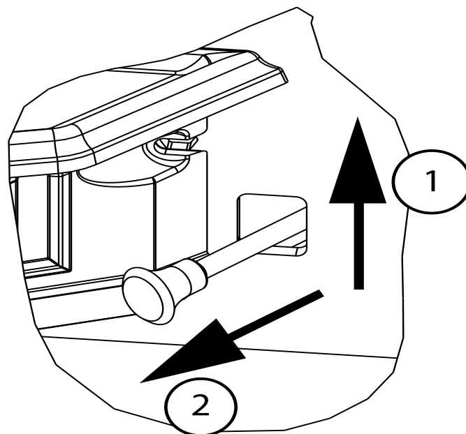
Figure 13.2 - Manual Timer Over-Ride
