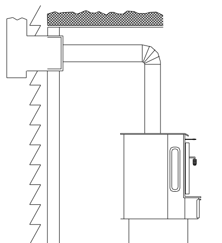
FIGURE 9 - INSTALLATION INTO A FACTORY BUILT CHIMNEY
