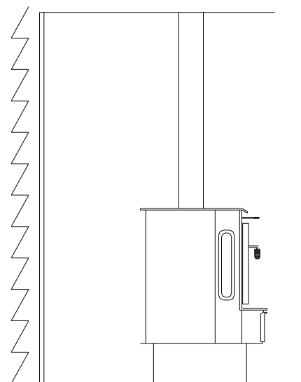
FIGURE 8 - INSTALLATION INTO A MASONRY FLUE
