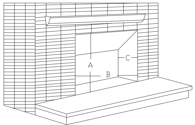
FIGURE 2 Fireplace Dimensions (Minimum)
