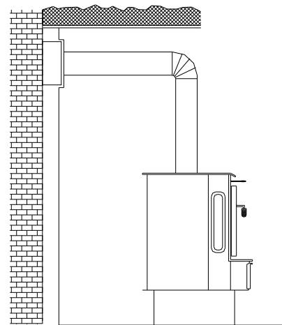
FIGURE 8 - INSTALLATION INTO A MASONRY FLUE
